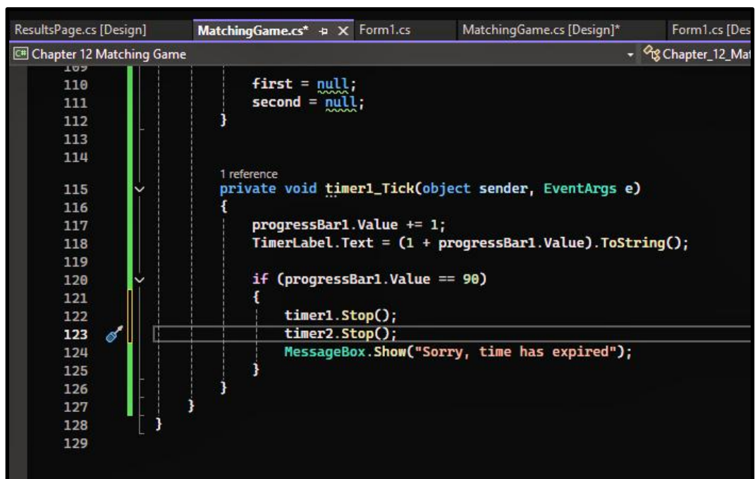
Figure 12B.8: timer1_Tick
