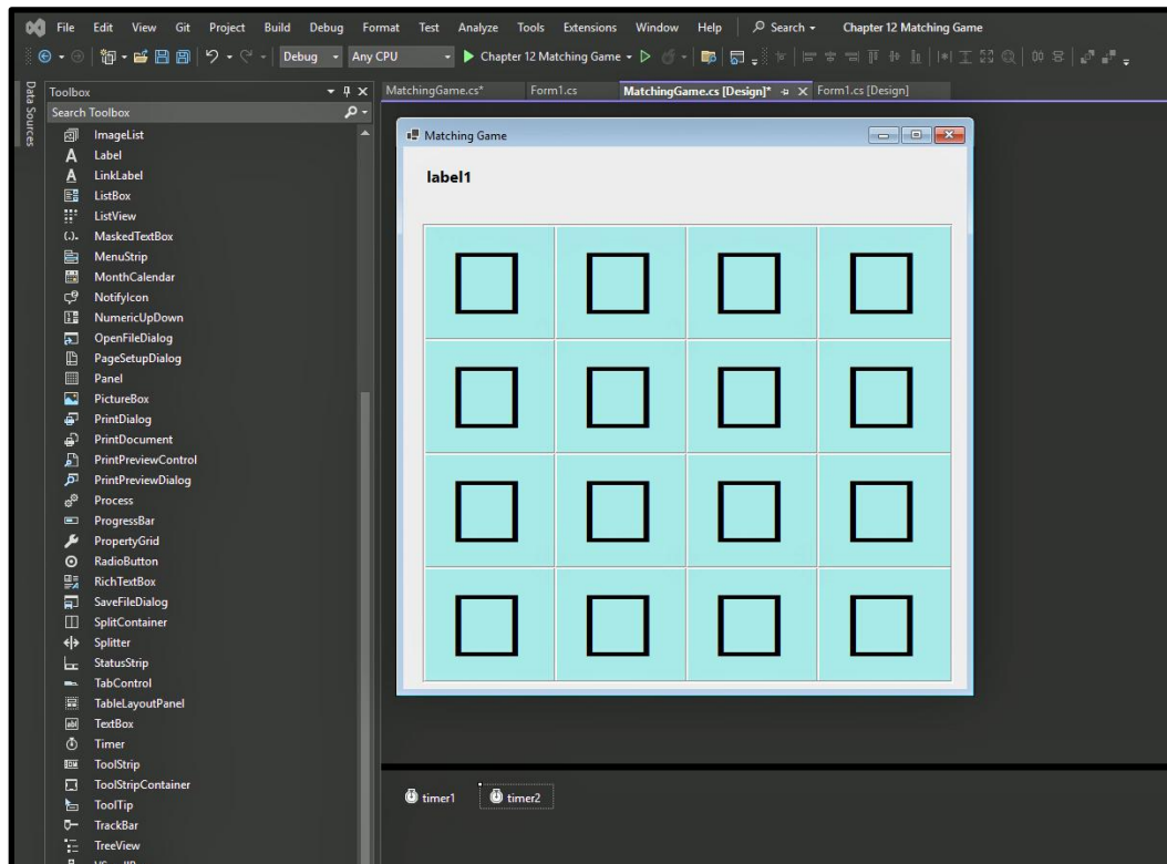
Figure 12B.4: Timers
