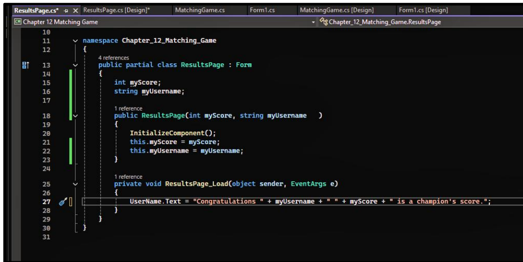
Figure 12B.12: ResultsPage_Load
